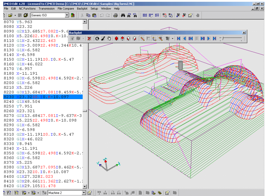
Cimco Edit with forward and backward toolpath simulation
